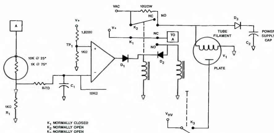
Figure 1. Self-heating properties of thermistors can be used to form time-delay circuits. In this example, the cathode is warmed before applying plate voltage and protects cold cathode from inrush current.
