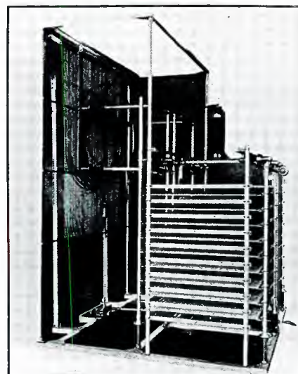
A portion of the WLW power amplifier tank circuit partially assembled. The 500kW transmitter used three such units.
