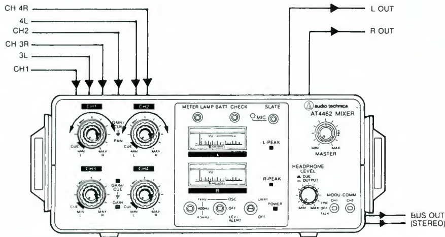
Figure 2. The mixer can be configured in three basic configurations: 4 × 2 (shown here), 6 × 1 or 4 × 1 with 2-way intercom.
