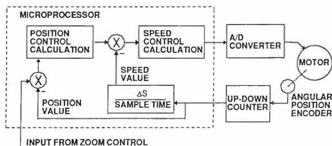
Figure 3. A motor control circuit for a microprocessor-controlled zoom lens.
