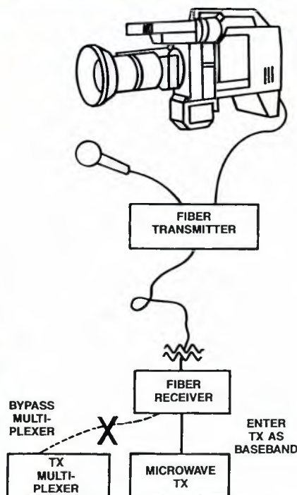
Figure 2. User-adjustable audio subcarrier frequencies on an advanced fiber-optic system allow video and audio signals to be transmitted in a baseband format from the camera into the station. This eliminates many conversion steps, greatly reducing noise degradation of the microwave signal.
