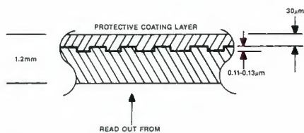
Figure 1. Cross section of CD showing the relatively thin upper coating. This layer can be depressed into the aluminum data area easily by pressing with a ball-point pen or sharp object.
