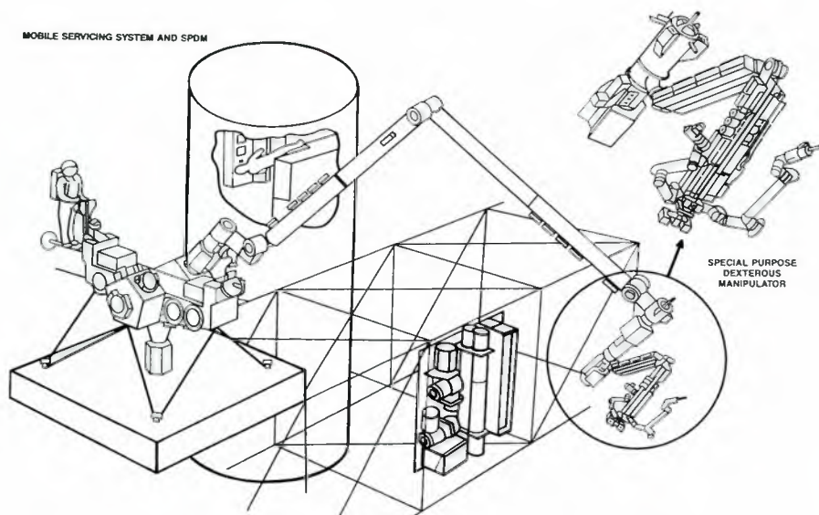
Figure 1. Special-Purpose Dexterous Manipulator is shown deployed on a shuttlelike arm, a part of the Flight Telerobotic Servicer system.
